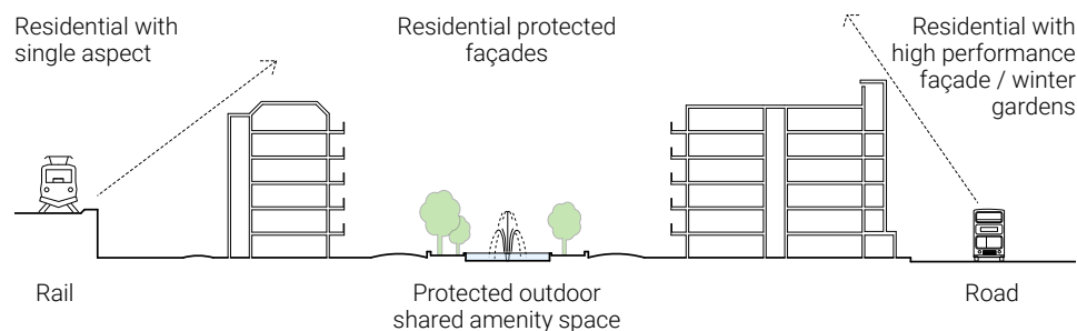
Figure 5. Noise mitigation measures through landscaping, site and building layout: noise from rail and road is buffered by the taller buildings, protecting the dwellings and landscaped areas on the other side (provided by Studio Partington).
